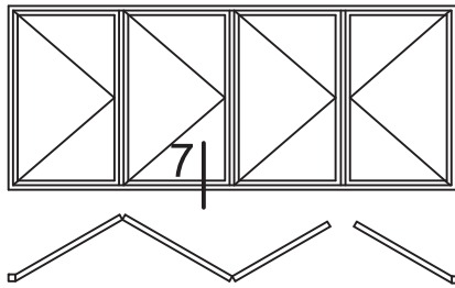
KATLANIR SÜRME KAPI Folding Sliding System Detail
