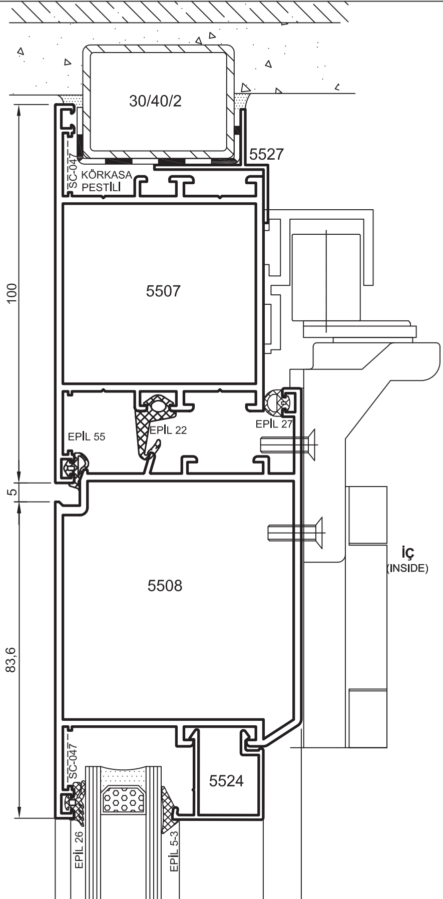
KATLANIR SÜRME KAPI Folding Sliding System Detail
