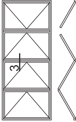
KATLANIR SÜRME KAPI Folding Sliding System Detail
