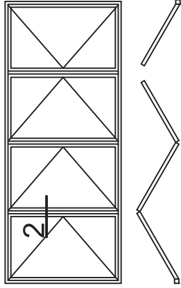
KATLANIR SÜRME KAPI Folding Sliding System Detail
